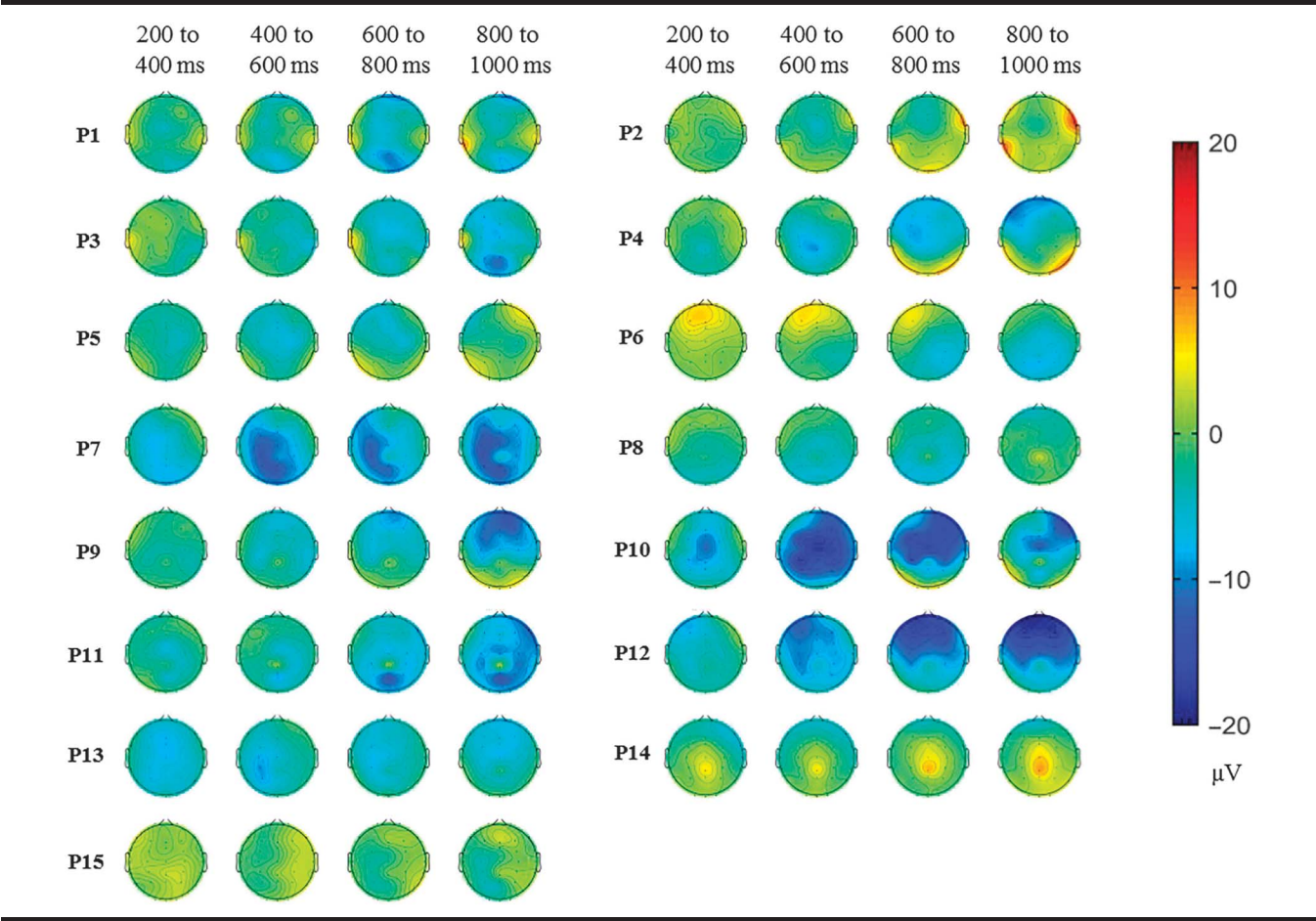
Figure 4. Experiment 1 (word pairs paradigm) individual topographic maps of the N400 effect (unrelated minus related condition) for 200-ms time windows from 200 to 1,000 ms after target onset for Neuroscan. Red areas indicate a more negative-going response for the related condition, and blue areas indicate a more negative-going response for the unrelated condition. The topography of the N400 effect varied across individuals. P = participant.
