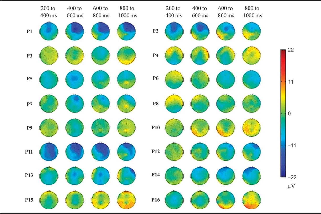
Figure 10. Experiment 2 (sentence paradigm) individual participant topographic maps of the N400 effect (incongruent minus congruent condition) for 200-ms time windows from 200 to 1,000 ms after target onset for Neuroscan. Red areas indicate a more negative-going response for the congruent condition, and blue areas indicate a more negative-going response for the incongruent condition. The N400 effect location was variable across individuals. P = participant.
