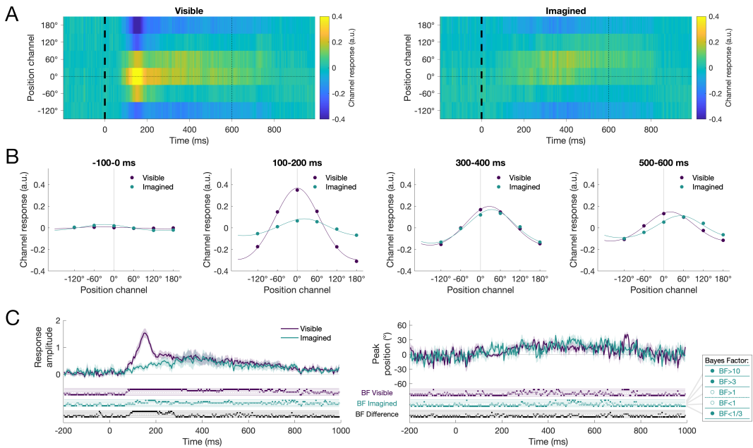
FIGURE 7 | Position response profiles for visible and imagined stimuli using encoding models trained on the random pattern estimator stimuli. A) Activations of each encoding position channel for visible and imagined stimuli, plotted as relationship to the presented stimulus position. For the visible and imagined conditions, there was higher activation for position channels closer to the correct position ( 0^\circ ), indicating that the neural representation of stimulus position was captured by the encoding model. B) Model fitting of channel responses for some representative time periods show the emergence of spatial information over time, with a shift towards the next stimulus position. C) Parameters of the model fits over time. Left: Response amplitude at each time point for visible and imagined stimuli. There was reliable spatial signal for both conditions, but the temporal dynamics varied. Right: Peak position for the model fit generally reflected a peak at 0^\circ for visible and imagined stimuli, although after 250ms there was some evidence of positive shifts towards the upcoming stimulus position.
