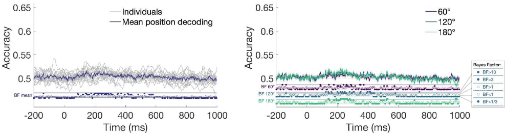
FIGURES S 3.1 Bayes Factors (BFs) associated with position decoding accuracy as a function of time, plotted on log scale. A) Visible stimuli. B) Imagined stimuli. Left plots show BFs associated with decoding all stimulus positions, and right plots show BFs associated with decoding according to the angular distance between position pairs.
